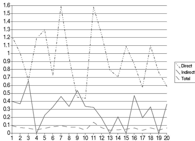
Figure 1: Effect of the presence of anomalies over Total and Partial Log-likelihoods on a set of 20 variable. The X axis shows the attribute that was modified. The Y axis shows the difference in log-likelihood between original and modified values divided by the original value.
